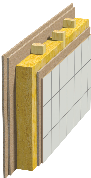
Fig. 3 Internal wall Offset wood studs on wood sill. Double boards.
