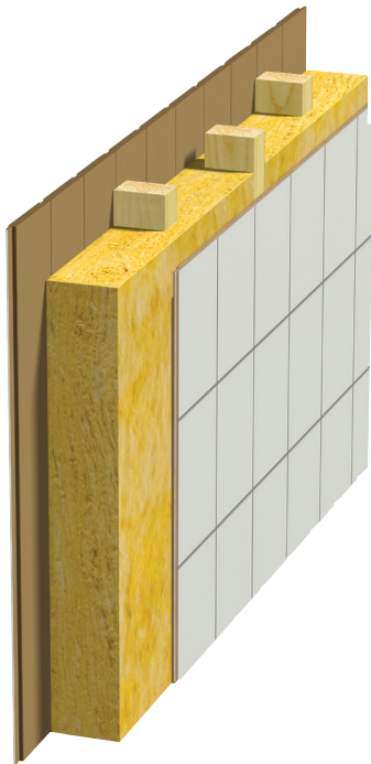
Fig. 2 Internal wall Offset wood studs on wood sill. Single board.
