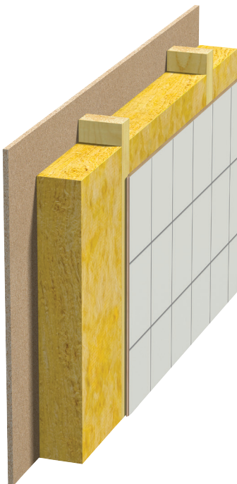
Fig. 1 Internal wall All through wood studs. Single board.
