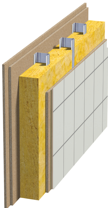
Fig. 6 Internal wall Offset steel studs. Double boards.
