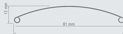
Slat cross-section
